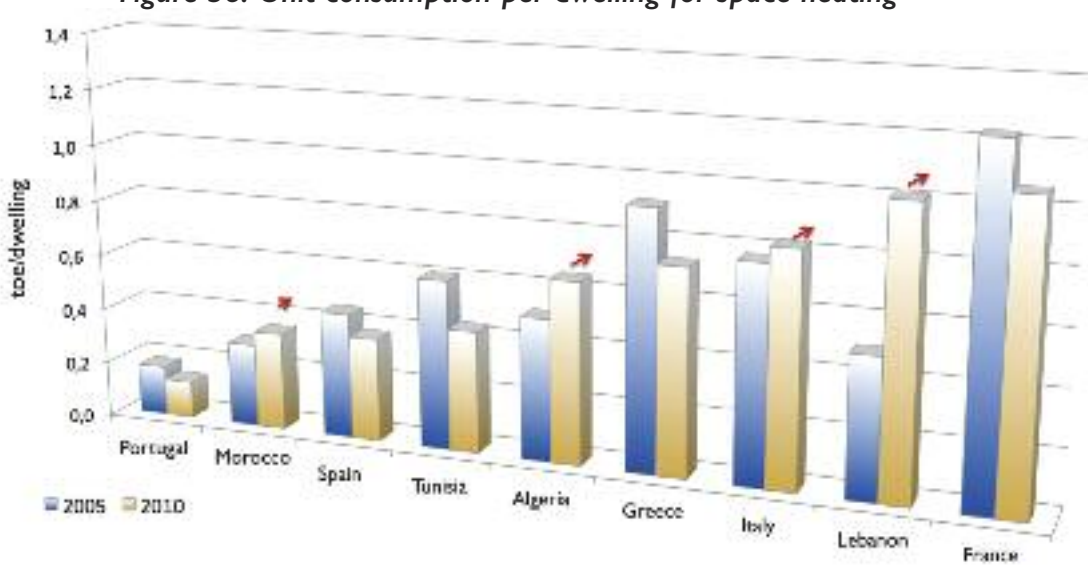
Figure 38: Unit consumption per dwelling for space heating 21
